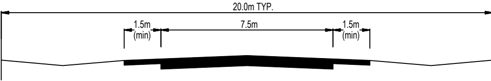
LOW DENSITY RESIDENTIAL COLLECTOR ROAD
