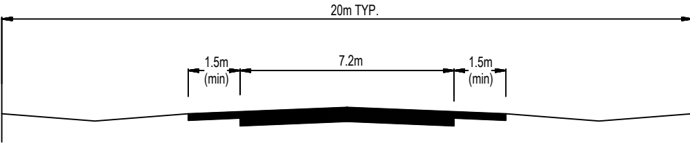
RURAL LIVING COLLECTOR ROAD
