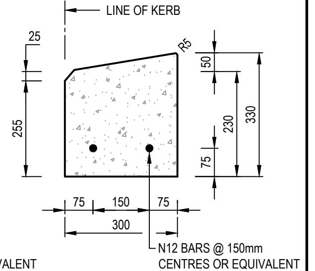
MOUNTABLE KERB (INDUSTRIAL) ⑤
