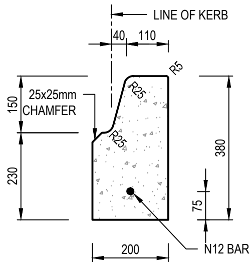
150mm BARRIER KERB ONLY (INDUSTRIAL) ①
