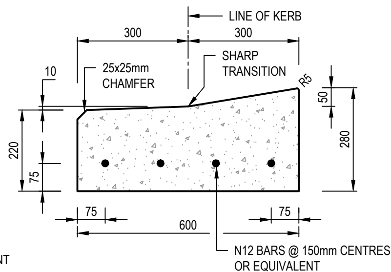
MOUNTABLE KERB AND TRAY (INDUSTRIAL) ⑦
