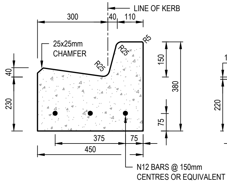
150mm BARRIER KERB AND WATER TABLE (INDUSTRIAL) ②
