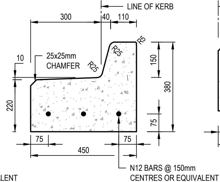
150mm BARRIER KERB AND TRAY (INDUSTRIAL) ③
